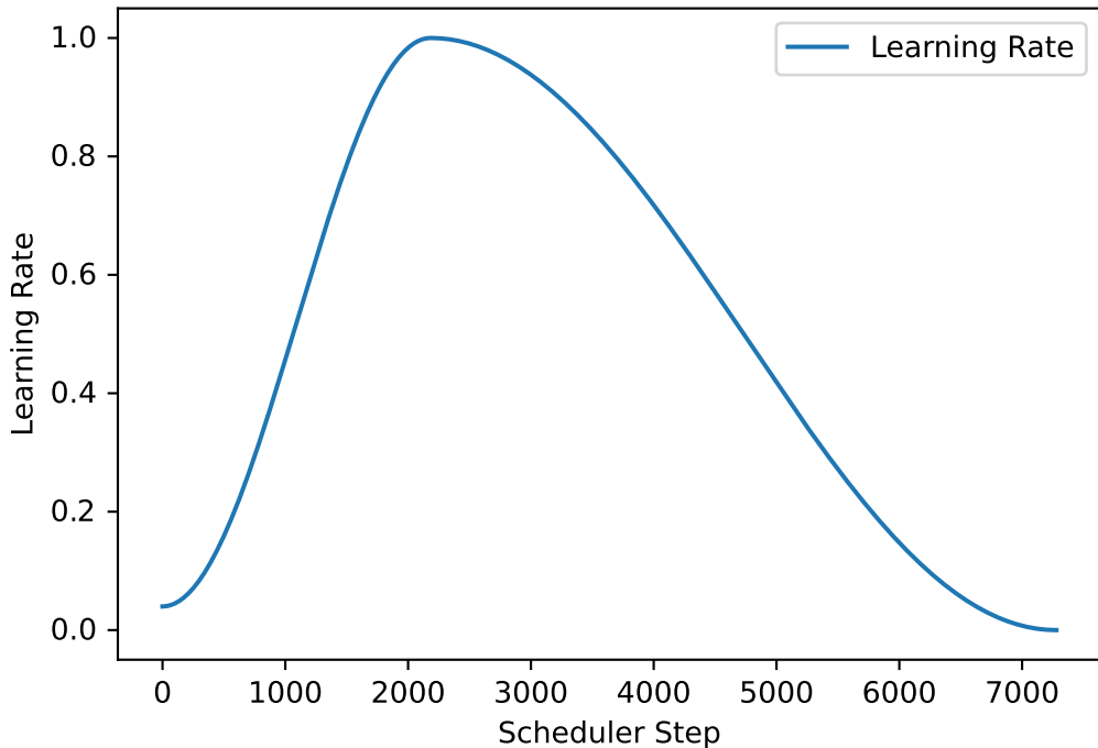
\times 10^{-4} MMPD_5FOLD_physnet_fold1 LR Schedule
