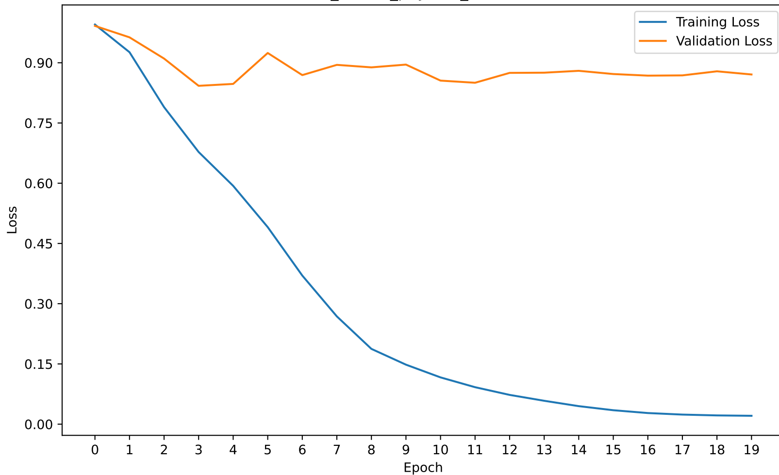
MMPD_5FOLD_physnet_fold1 Losses
