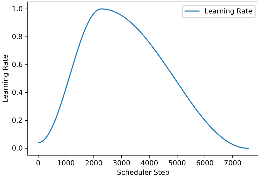
\times 10^{-4} MMPD_5FOLD_physnet_fold3 LR Schedule
