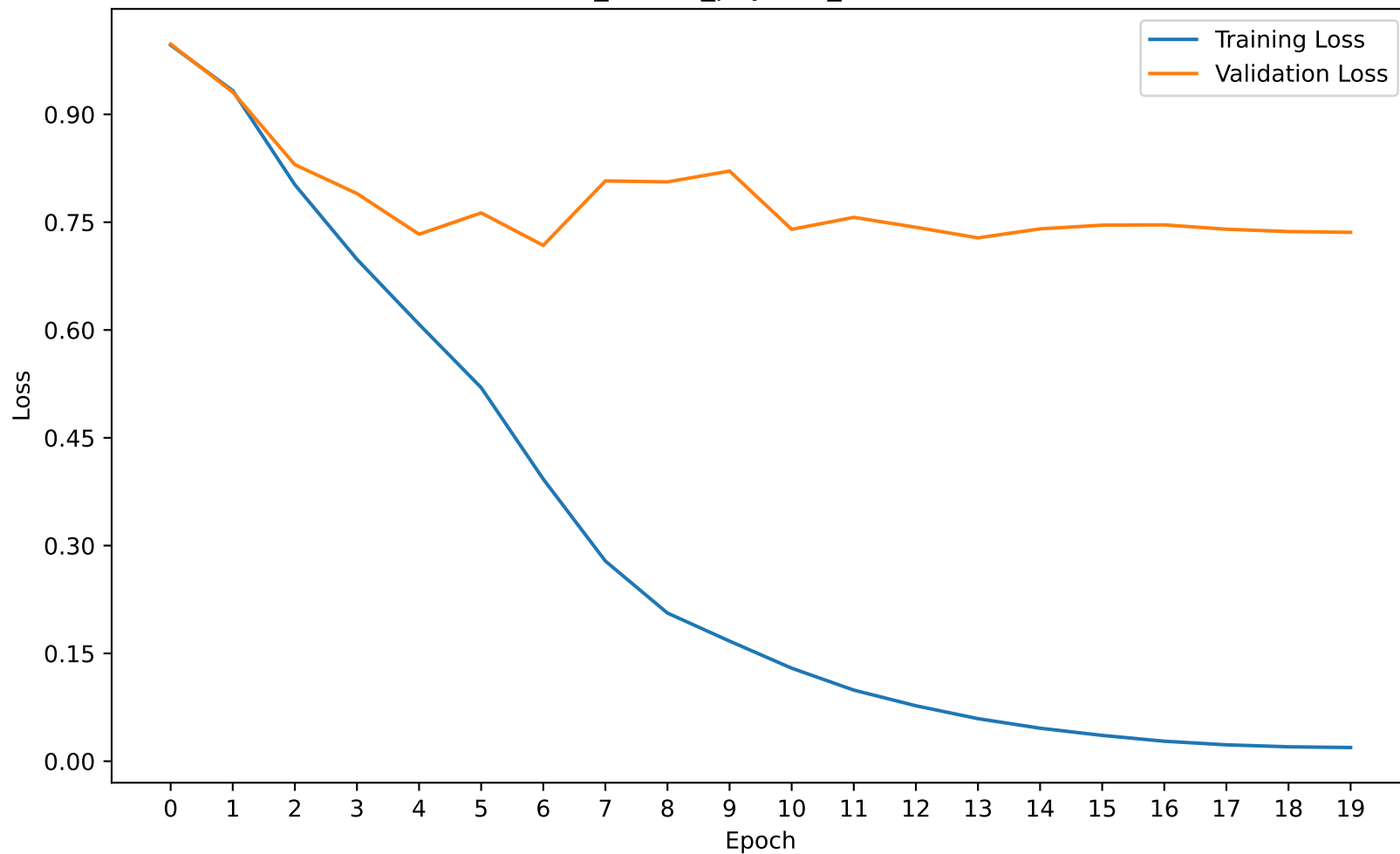
MMPD_5FOLD_physnet_fold3 Losses
