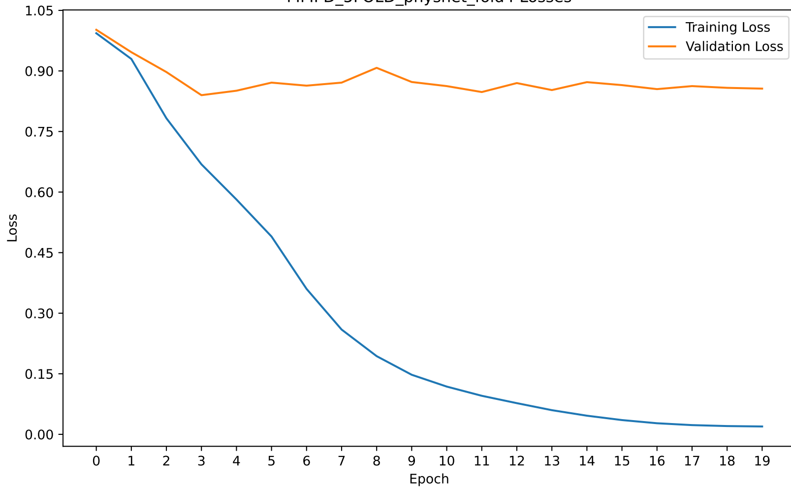
MMPD_5FOLD_physnet_fold4 Losses
