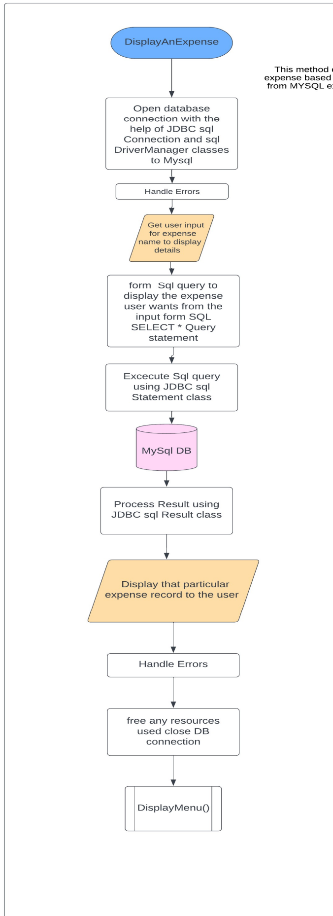
Flow Chart for Method :DisplayAnExpense
