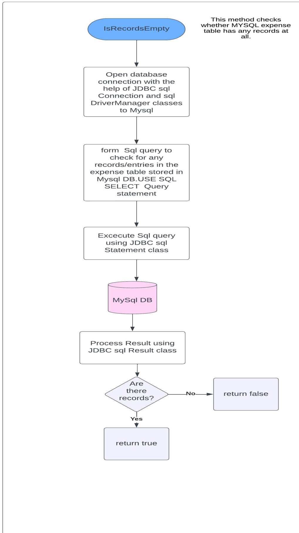
Flow Chart for Method :IsRecordsEmpty
