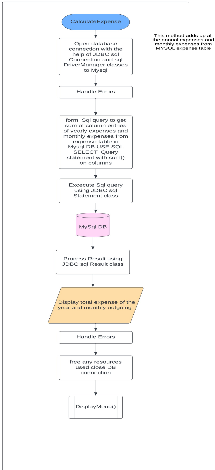
Flow Chart for Method :CalculateExpense
