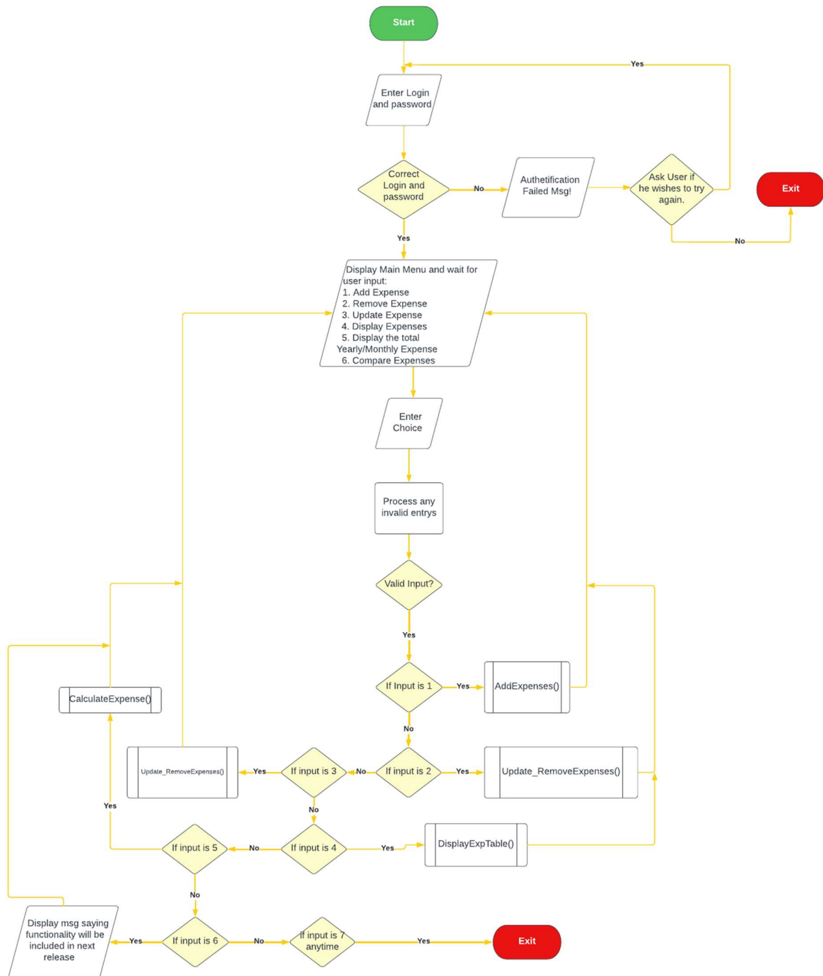
INITIAL FLOW CHART FOR EMS BEFORE CLIENT's REQUEST FOR CHANGE
