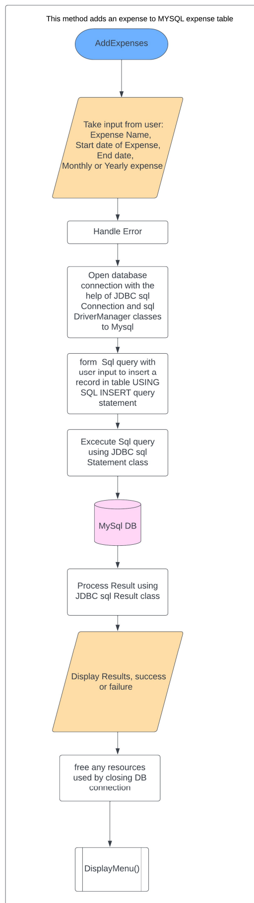
Flow Chart for Method :AddExpense
