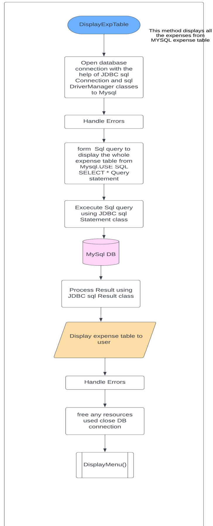
Flow Chart for Method :DisplayExpTable
