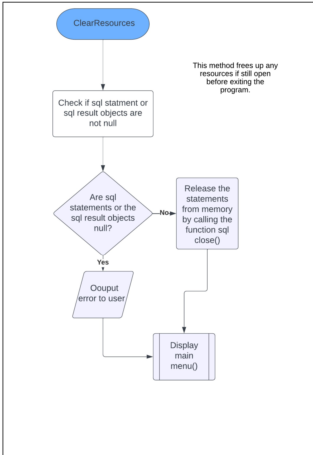
Flow Chart for Method :ClearReasources
