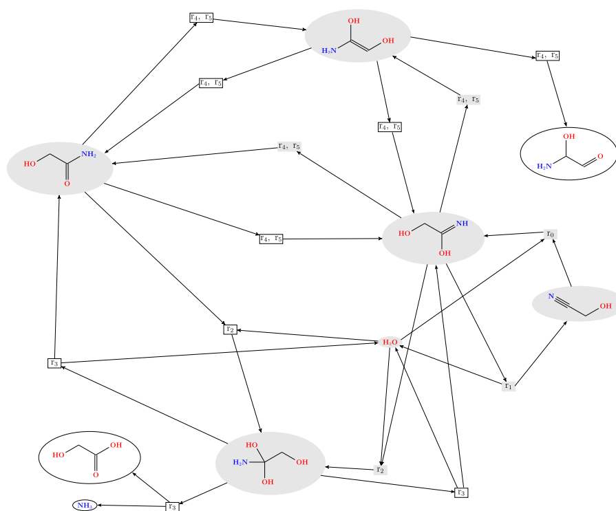
Figure 3.8: The reaction network (with 9 molecules and 14 reactions) after three recursive applications of the graph transformation rules with the 3-cycles filtered out. The part of the network already generated previously has been shaded.
