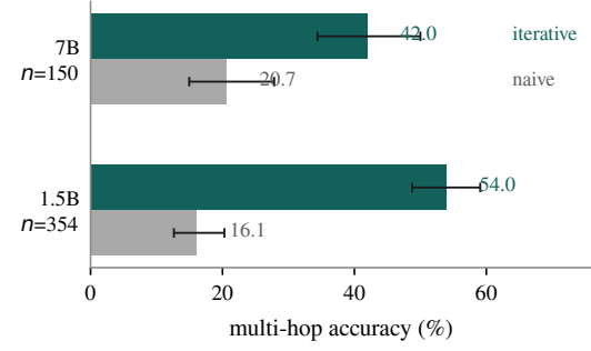
Figure 3: Iterative decomposition versus naive single-shot on MQuAKE-CF after the per-hop fallback fix, with 95% Wilson intervals.
