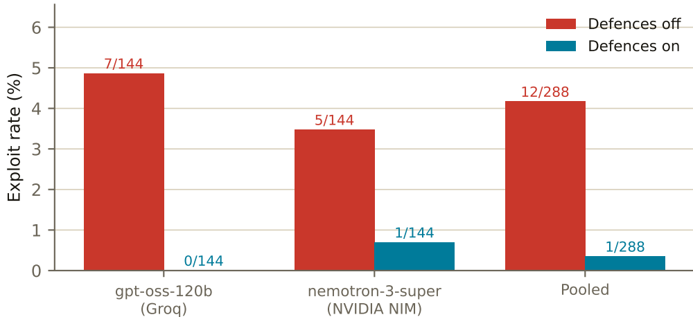
Indirect prompt injection, measured on two vendors
