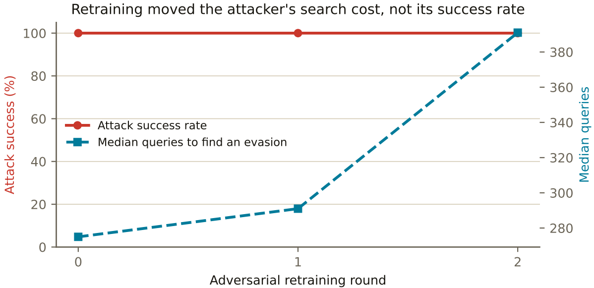
Figure 2: Attack success is flat at 100.0% across every round, while the search needed to reach it lengthens: median queries 275 \rightarrow 391. Sparsity is unchanged over the same rounds (4.12 \rightarrow 4.03), so the honest reading is that retraining made evasions harder to find rather than structurally more costly. A defence that raises the price of an attack without preventing it is a real outcome, and reporting it as a fall in success rate would have been the easier story.
