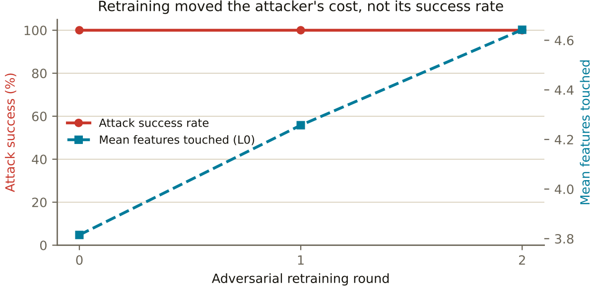
Figure 2: Attack success is flat at 100.0% across every round. The attacker’s cost is not: it touches more features and spends more queries each round to find an evasion that still works. A defence that raises the price of an attack without preventing it is a real outcome, and reporting it as a fall in success rate would have been the easier story.
