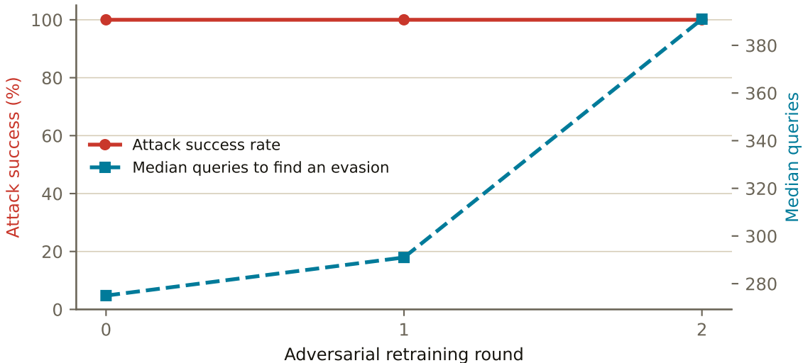
Retraining moved the attacker's search cost, not its success rate
