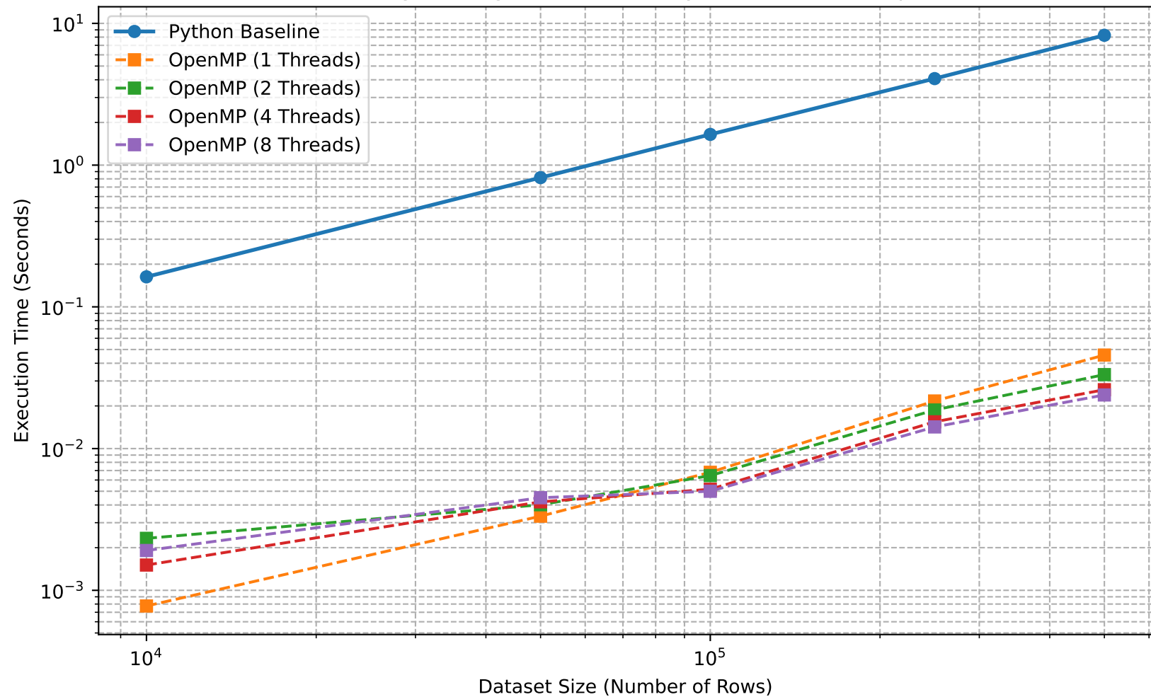
Feature Engineering Performance: Python vs Parallel OpenMP
