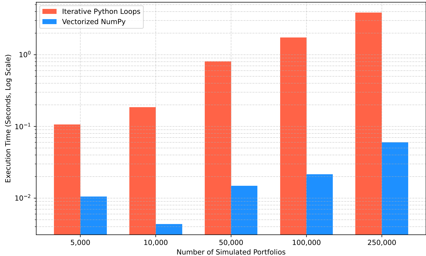
Monte Carlo Portfolio Optimization Speedup
