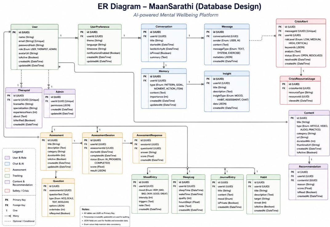
Figure 4.9 Entity-Relationship Diagram
