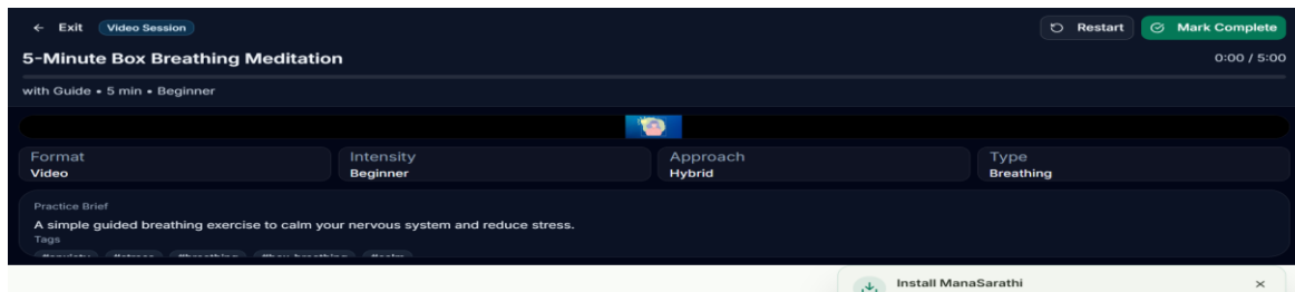
Figure 9.12 Practice Session
