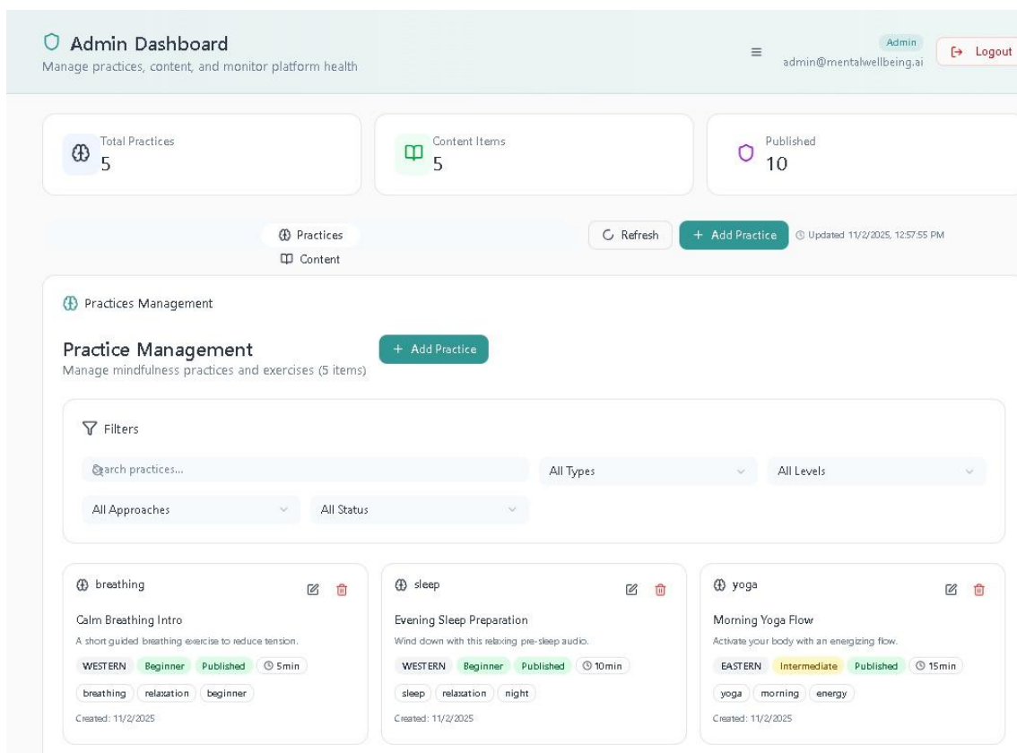
Figure 9.4 Admin Dashboard
