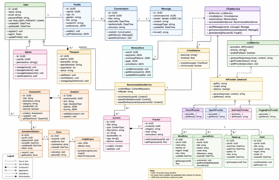
Figure 4.10 Class Diagram
