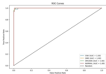
Fig. 7. DenseNet model ROC curve
