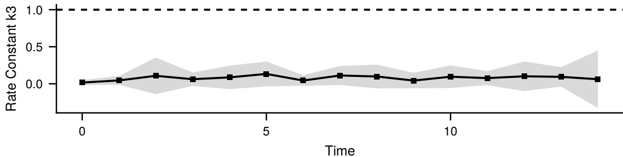
Reaction 3: [1, 0]
