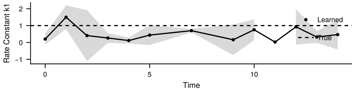
Reaction 1: [-1, 0]
