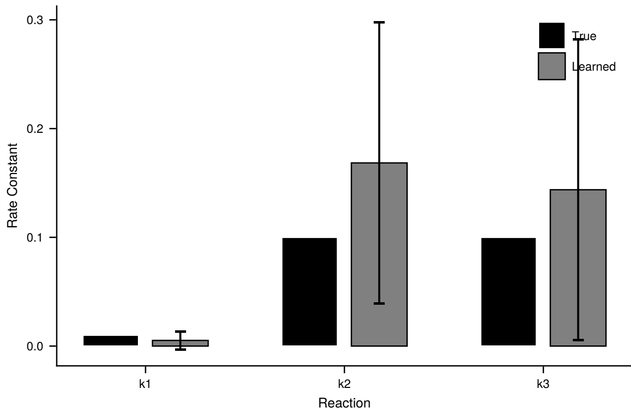
Final Learned vs True Rates
