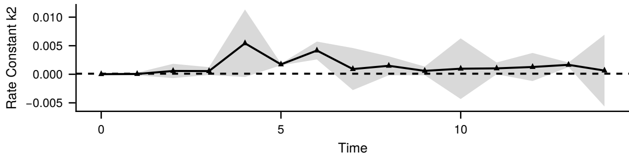
Reaction 2: [-1, 1]
