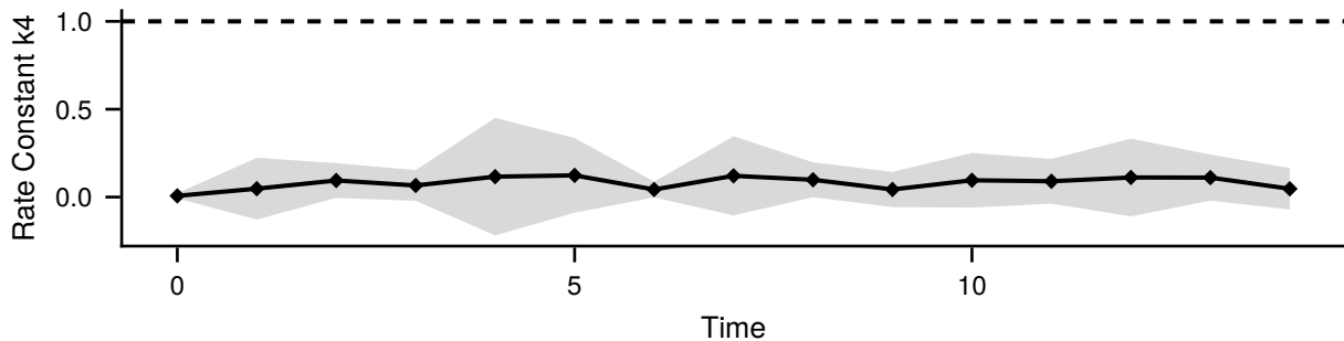
Reaction 4: [1, -1]
