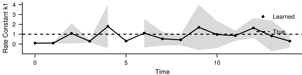
Reaction 1: [-1, 0]
