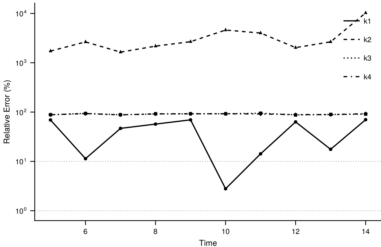
Rate Convergence
