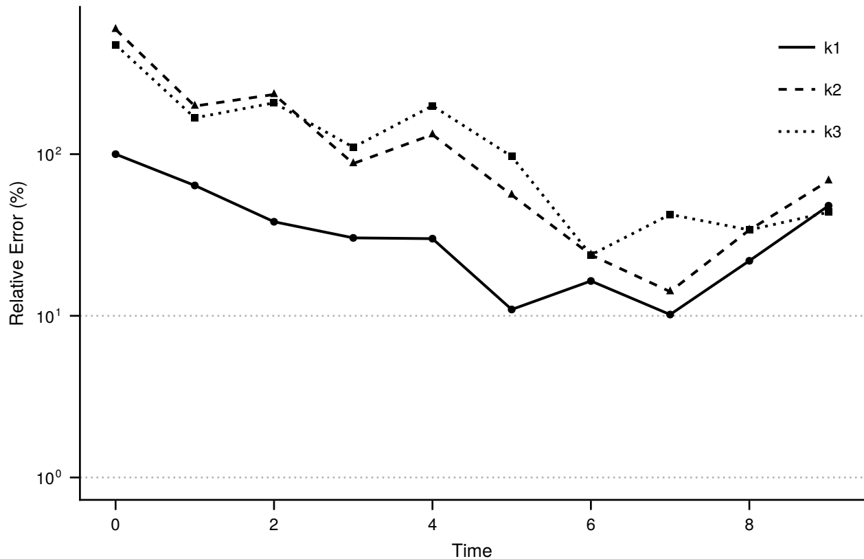
Rate Convergence
