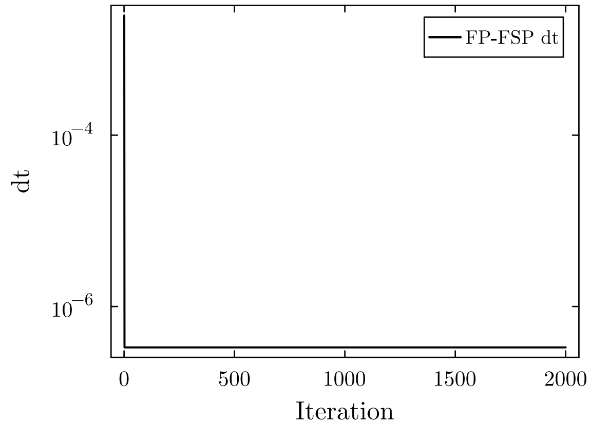
(a) FP-FSP time step
