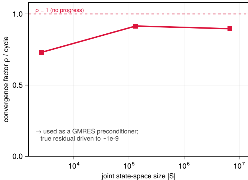
Standalone V-cycle stalls (smoother-limited)
