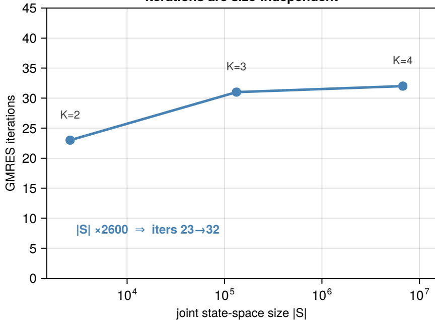
Iterations are size-independent
