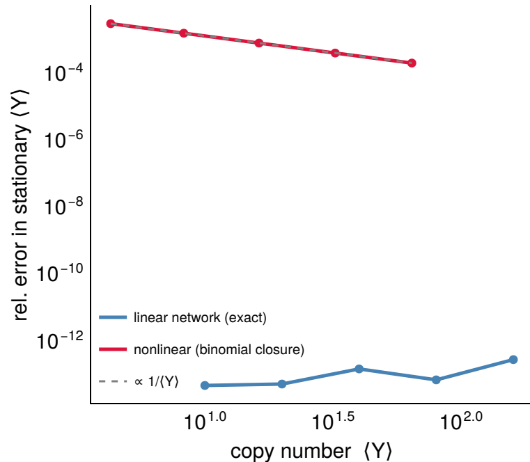
(a) closure error vs copy number
