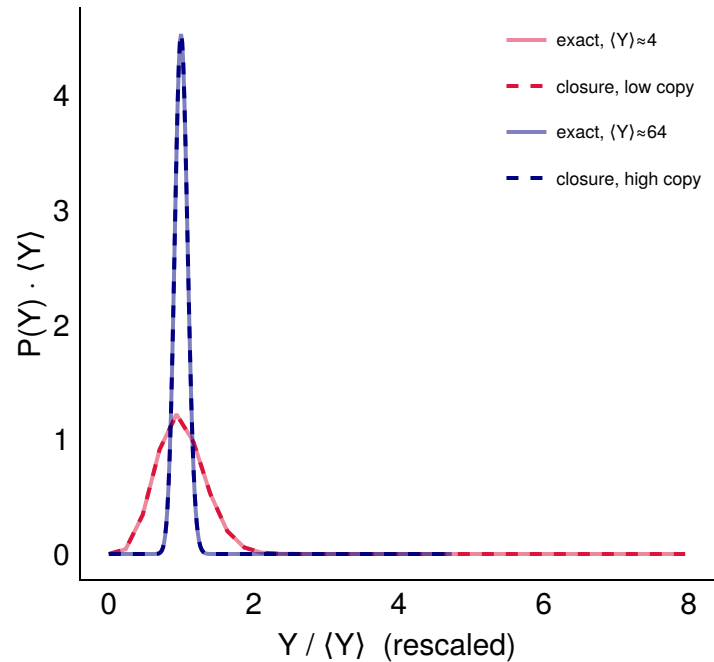
(b) coarse stationary: exact vs closure
