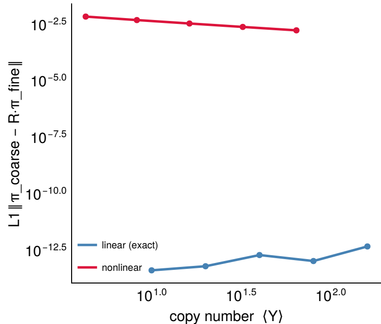
(c) distribution error vs copy number
