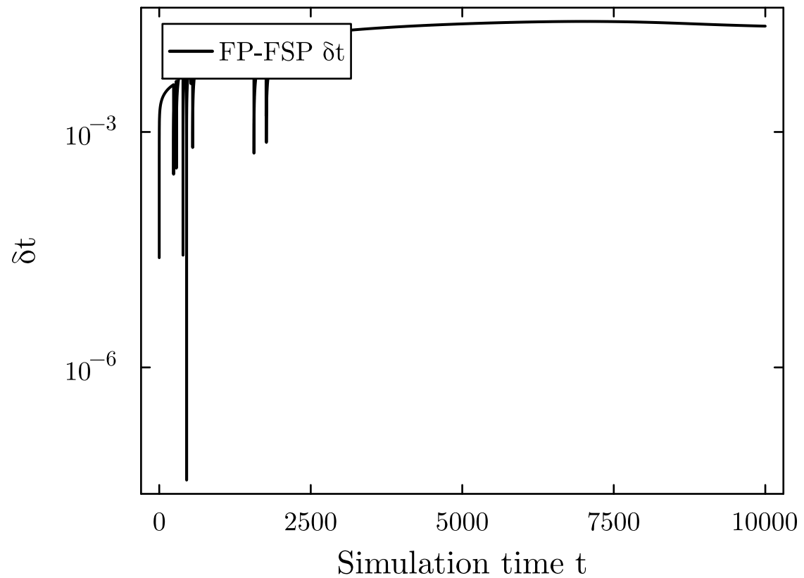
(a) FP-FSP: time step vs. time
