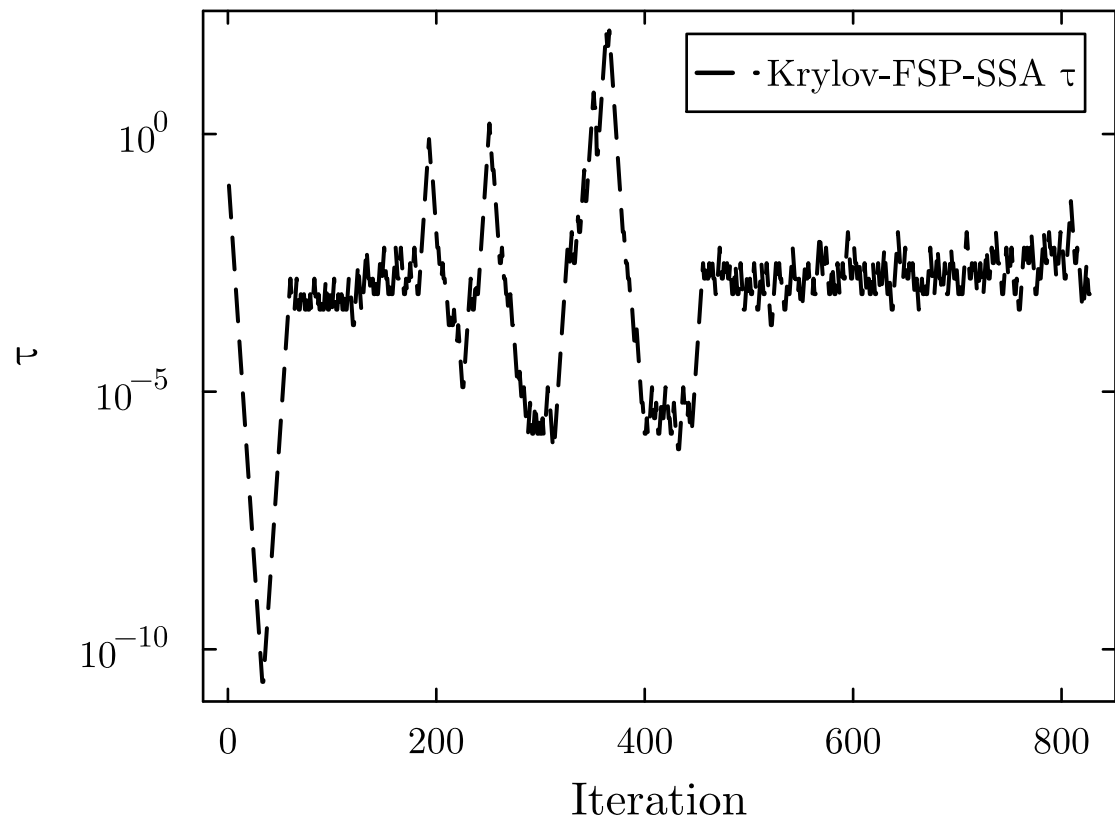
(b) Krylov-FSP-SSA: time step vs. iteration
