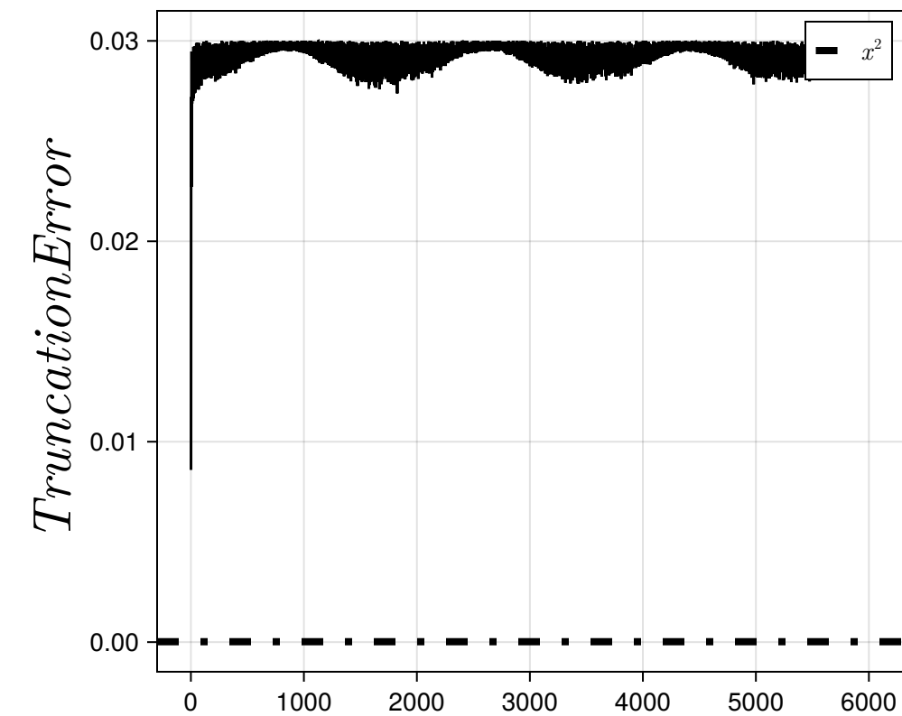
Michaelis Menten
