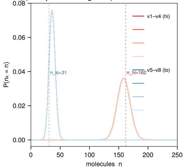
(b) K=8 per-voxel marginals (Binomial reconstruction)
