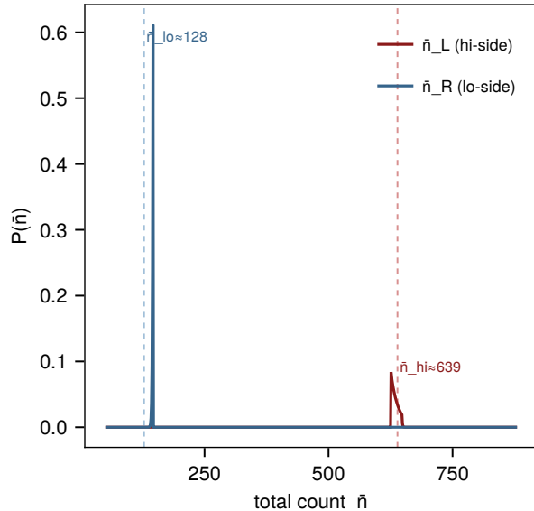
(a) K=2 coarse marginals at t=20
