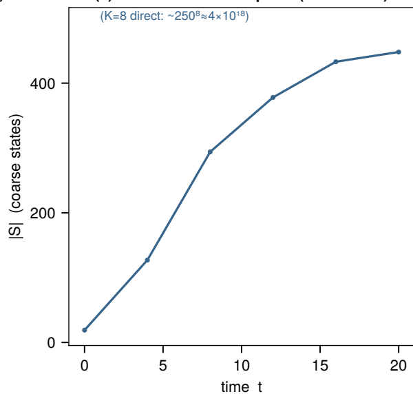
(c) K=2 coarse state-space (K=8 voxels)
