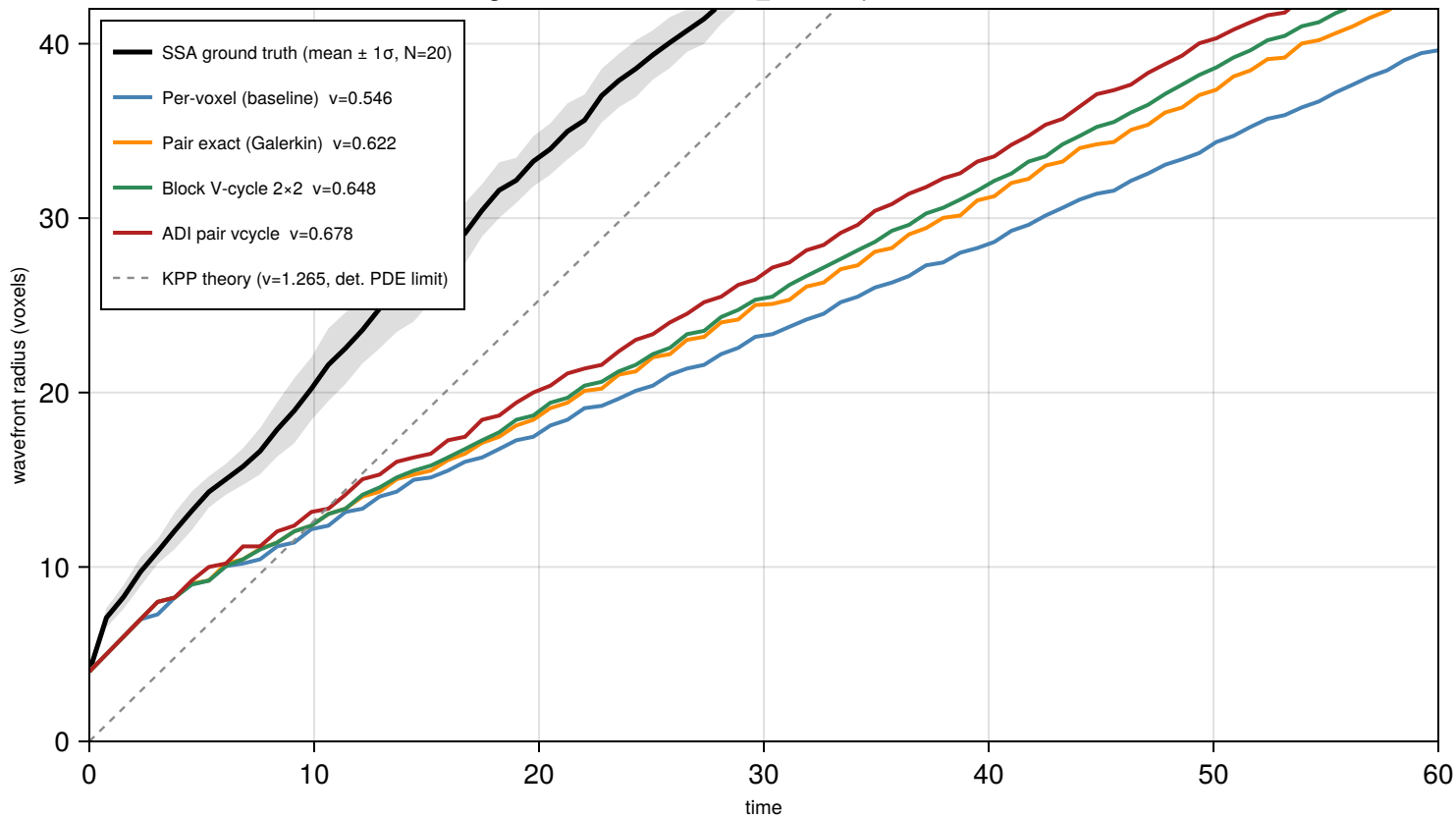
BranchingDeath RDME K=80×80 n_max=14 | wavefront radius vs time
