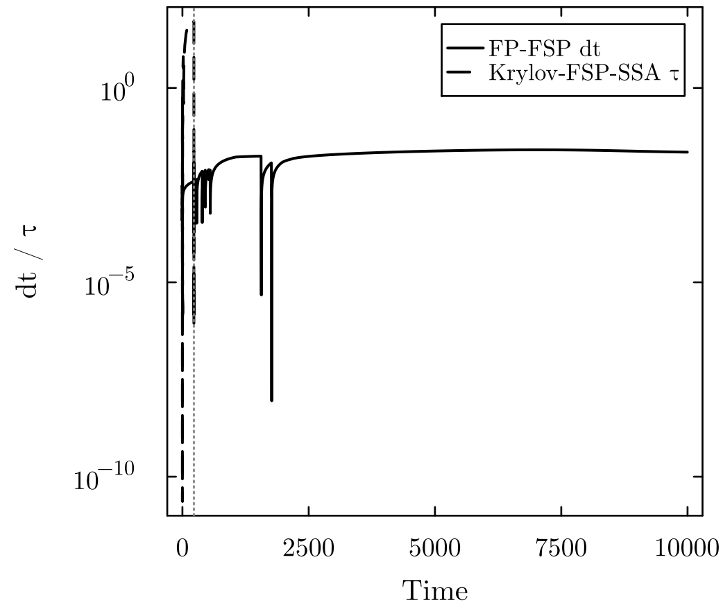
(c) Robertson
