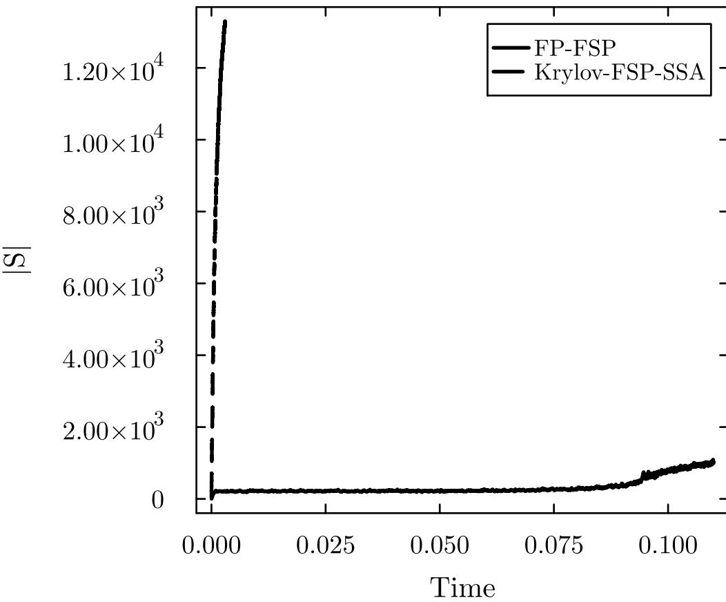
(a) Oregonator
