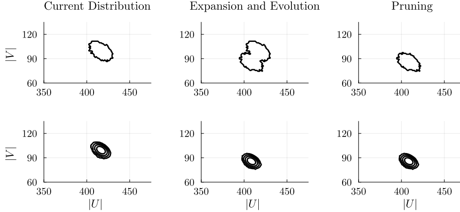
Fig. 1: Visualization of the adaptive FSP procedure (species U and V ) during a single time step in Algorithm 2.1. The top row shows the truncation boundary during the expand, evolve, and prune phases, while the bottom row shows the corresponding probability contours.
