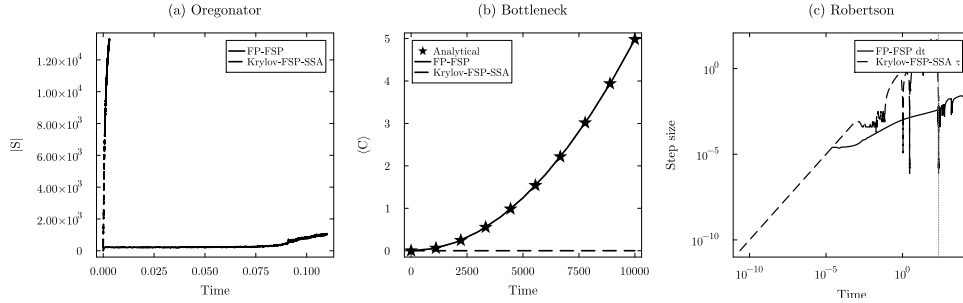
Fig. 12: FP-FSP (solid) vs. Krylov-FSP-SSA (dashed) on three benchmark systems. (a) Oregonator: state space size |S| vs. time. Krylov-FSP-SSA grows to \sim 13,300 states; FP-FSP stays below 1,100 via flux-based pruning. (b) Bottleneck ( A \rightarrow B \rightarrow B + C , t_f = 10^4 ): mean \langle C \rangle vs. time with analytical reference (dotted, stars). FP-FSP tracks the exact solution; Krylov-FSP-SSA underestimates by 40\times due to wavefront truncation. (c) Robertson ( t_f = 10^4 ): per-step \delta t (FP-FSP, solid, full horizon) and accepted \tau (Krylov-FSP-SSA, dashed; dotted vertical line marks t=228 where it stops) on a log scale. FP-FSP's non-monotonic \delta t reflects repeated autocatalytic bursts; Krylov-FSP-SSA incurs 67% rejections from k_2 = 3 \times 10^7 propensities and reaches only 2.3% of t_f .
