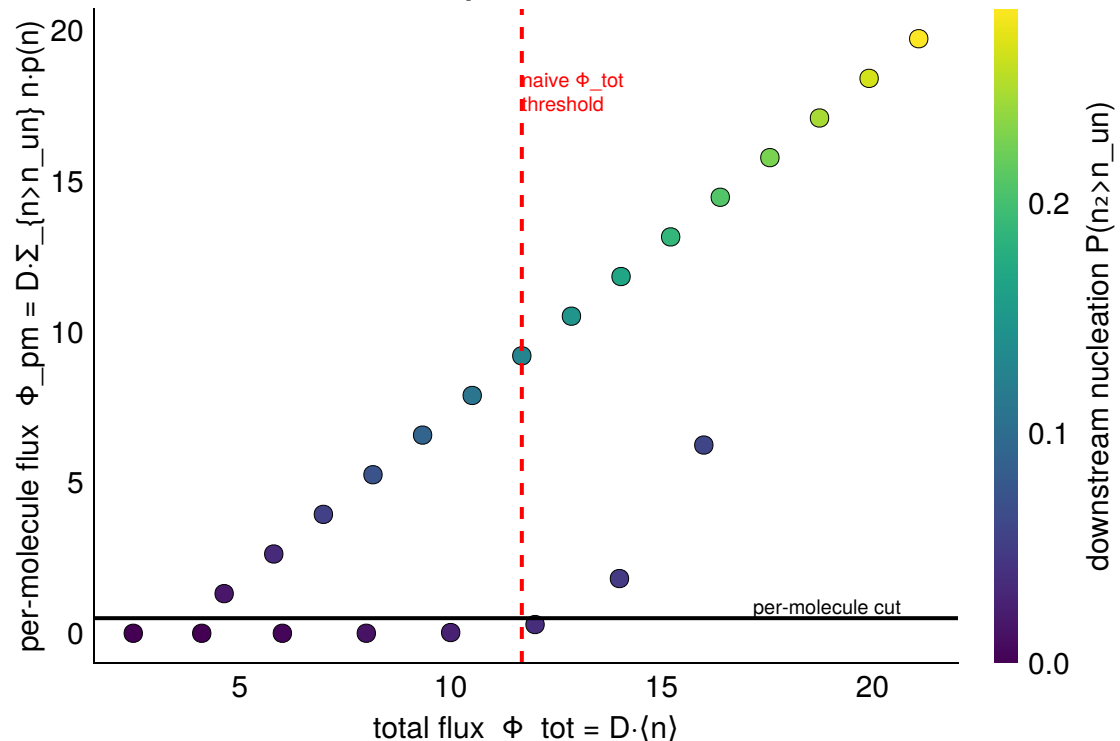
(b) activation decision plane (colour = true nucleation)
