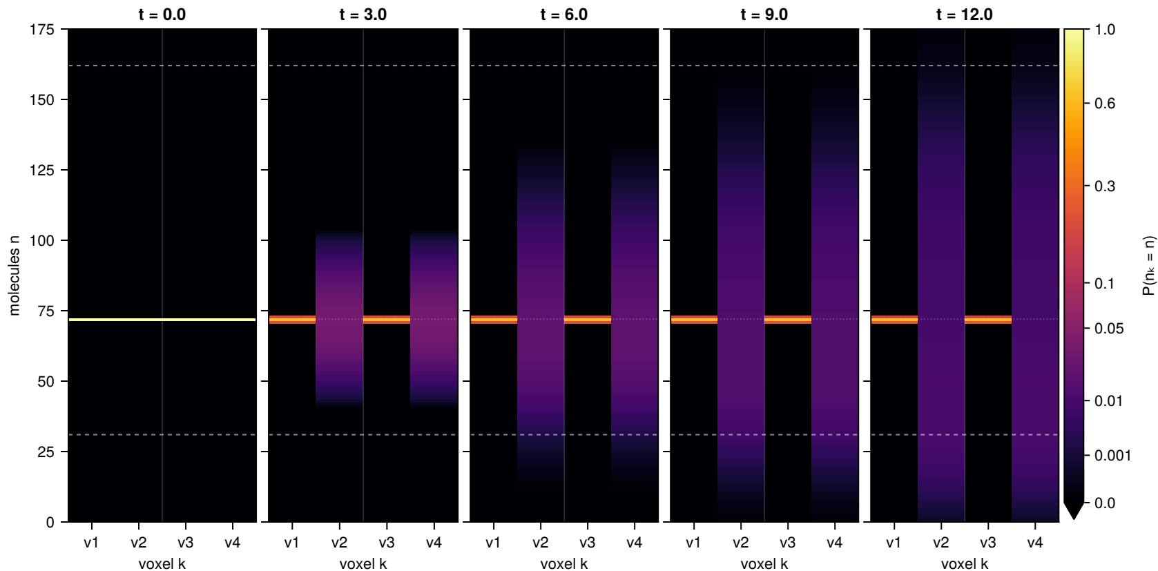
Schlögl RDME: K=4 voxels, D=5.0 — unstable IC ( n=72 ) splitting toward low ( n=31 ) and high ( n=162 ) [color: P(n_k=n)^{1/3} ]
