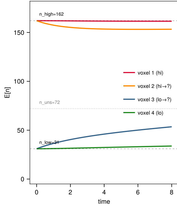
1. Mean-field ODE ( E[n \cdot (n-1)] \approx E[n]^2 : wrong for bistable)
