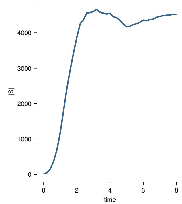
Multigrid FSP state space ( D=0.05 , prune=0.0001, expand=0, cr=1)
