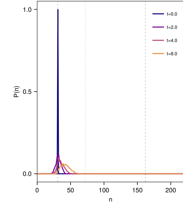
Multigrid FSP: P(n) at voxel 3 (lo→?)
