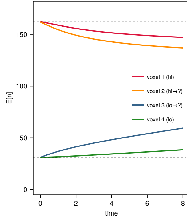
2. Per-voxel FSP + mean-field coupling (front mean \approx n_{\text{uns}} → injects unstable point into neighbours)
