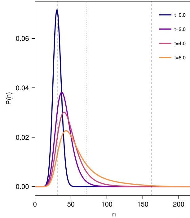
Per-voxel FSP: P(n) at voxel 3 (lo→?)
