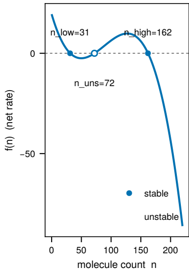
(a) Schlögl rate equation
