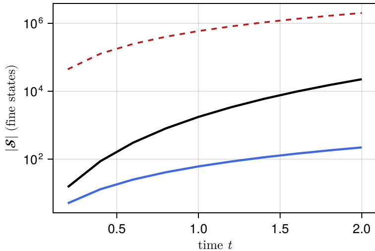
State space size
