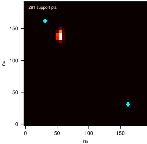
(a) FSP exact P(n_3, n_4) t=3
