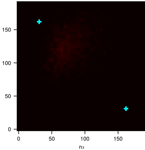
(b) SSA histogram N=10^3 t=3
