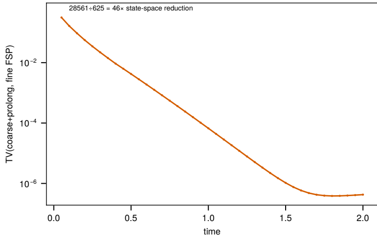
(b) Accuracy [coarse generator exact for linear networks]
