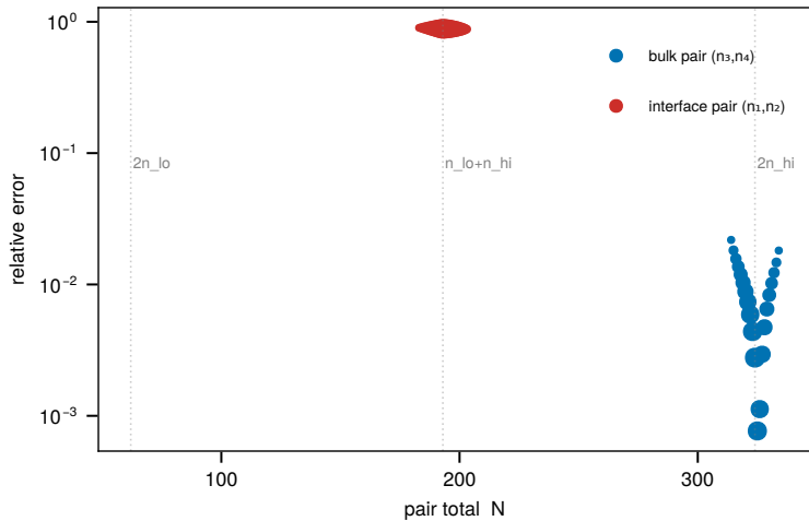
(a) Second factorial-moment closure error
