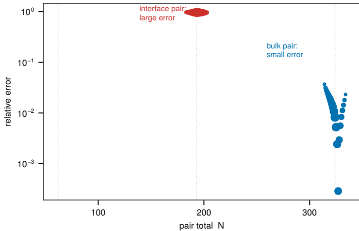
(b) Third factorial-moment closure error
