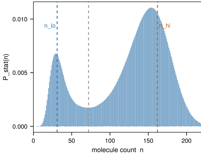
(b) Stationary distribution
