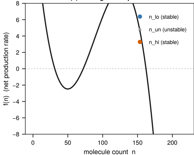
(a) Schlögl rate equation
