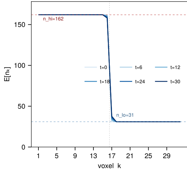
(a) Per-voxel mean: K=32 adaptive coarse
