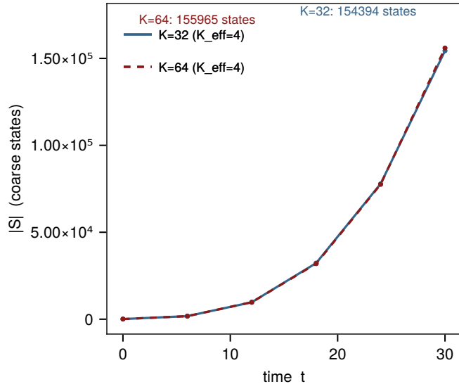
(b) State-space: K=32, K_eff=4 adaptive
