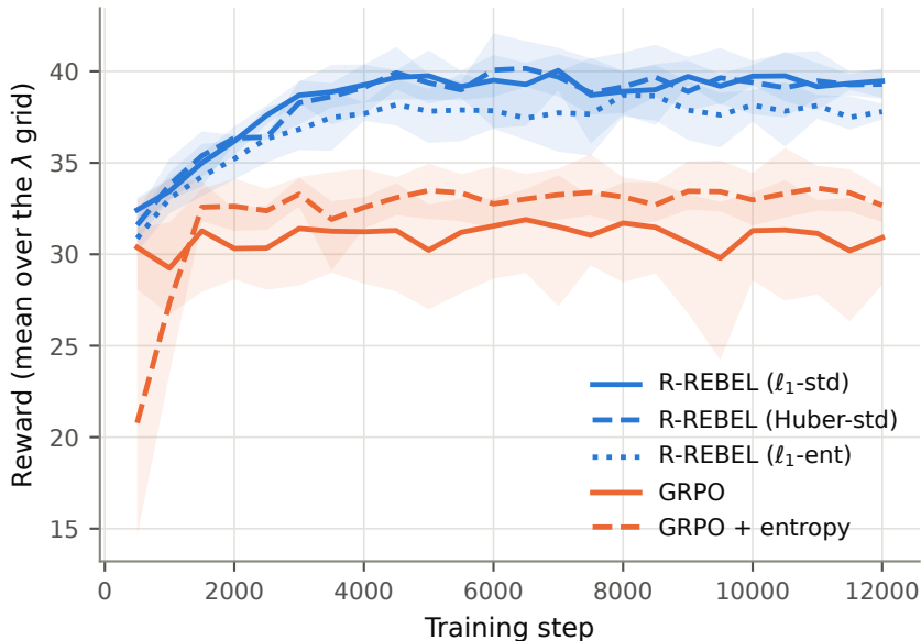
Learning curves (mean of 3 seeds, band = min-max)
