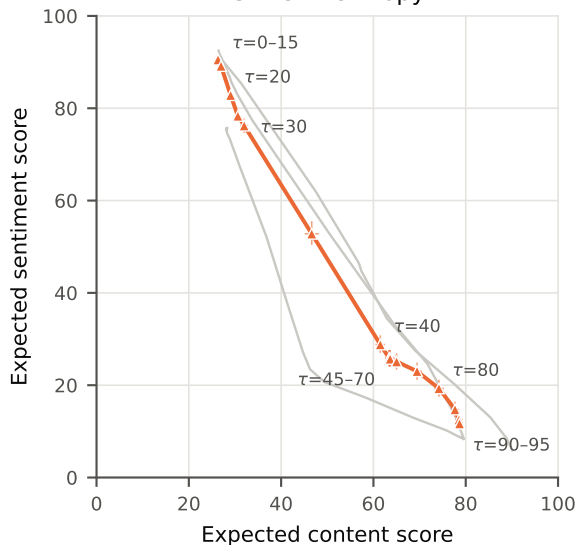
GRPO + entropy
