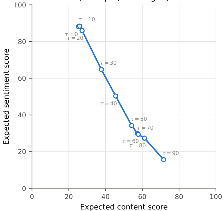
R-REBEL ( \ell_1 ) (test split, converged)
