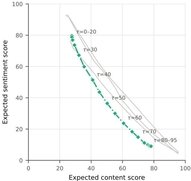
GRPO, base-LM reference
