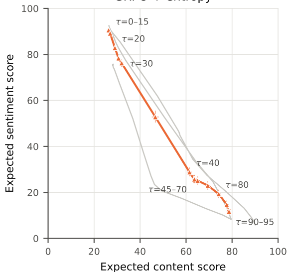
GRPO + entropy
