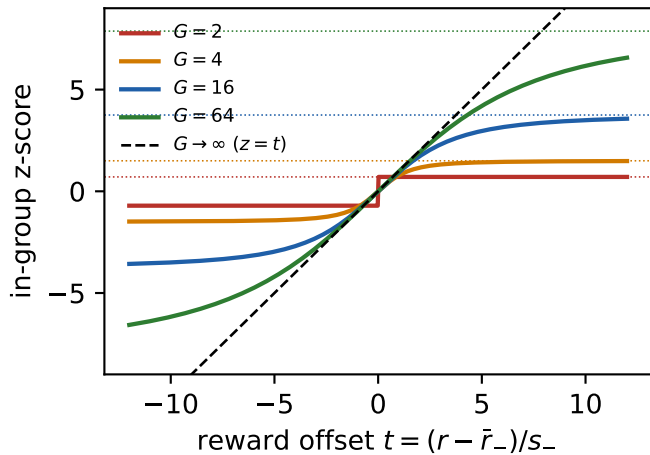
(a) soft clip at \pm(G - 1)/\sqrt{G}
