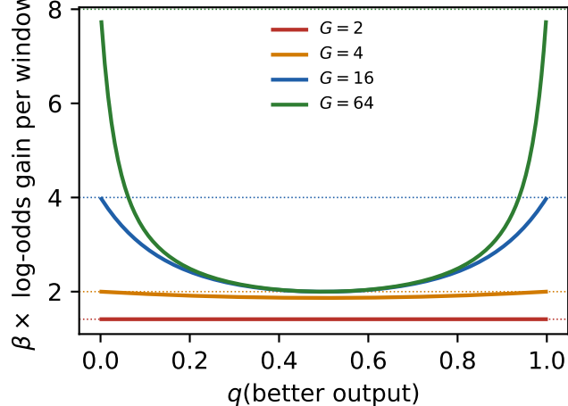
(b) binary rewards: gain \in [\sqrt{2}, \sqrt{G}]
