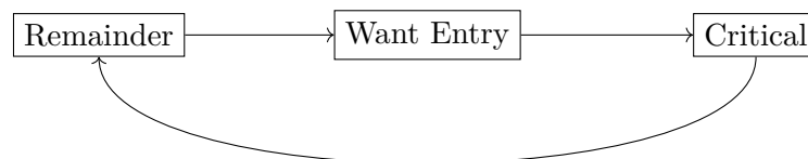
Figure 7.3: Peterson's Algorithm States
