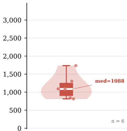
Figure 1 — Latency Distributions: Cold Start (top) vs. Warm Ping (bottom) Violin (KDE) + box (IQR) + jittered observations; independent y-axes per row
