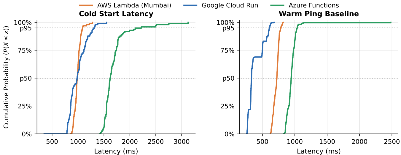
Figure 1 — Empirical Cumulative Distribution Functions (ECDF) [Domestic Mumbai Replication] Left: Cold Start Latency; Right: Warm Baseline (Dashed Lines: p50 and p95)
