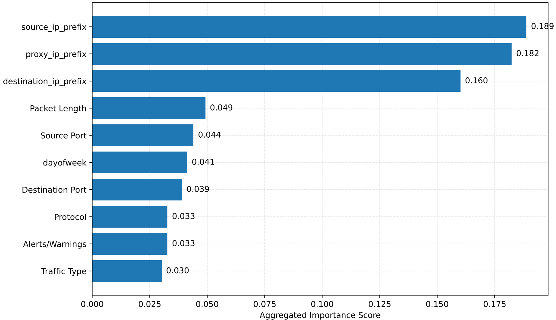
Figure 4. Top 10 Feature Importance Scores for Severity Level Classification
