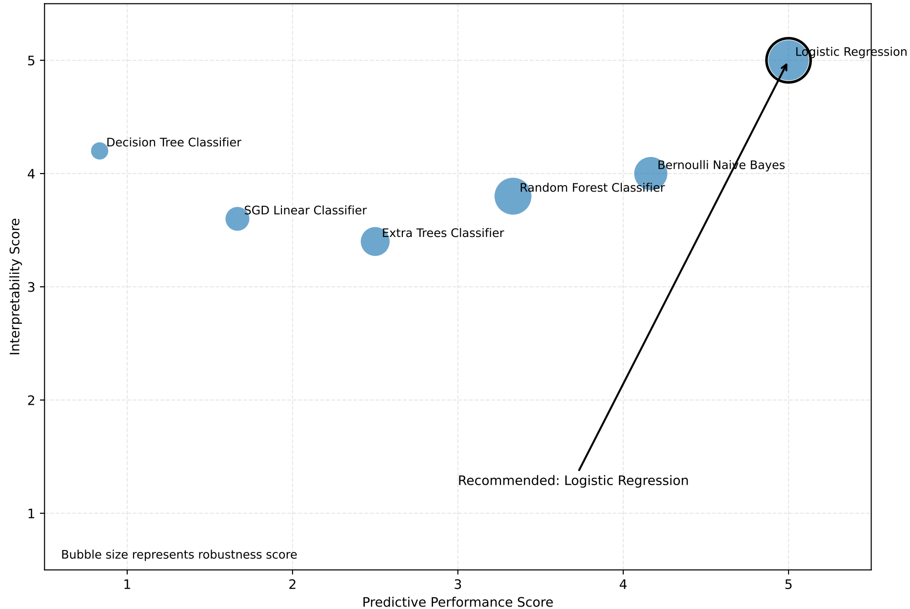
Figure 7. Final Trade-off Analysis for Severity Level Classifier Selection
