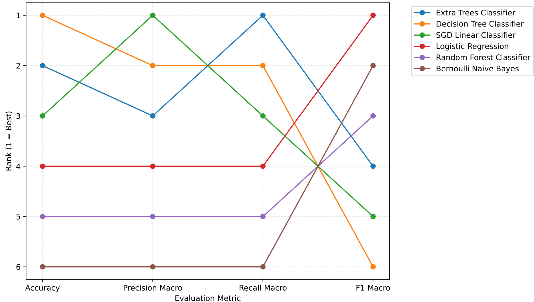
Figure 5. Variation in Model Rankings Across Evaluation Metrics
