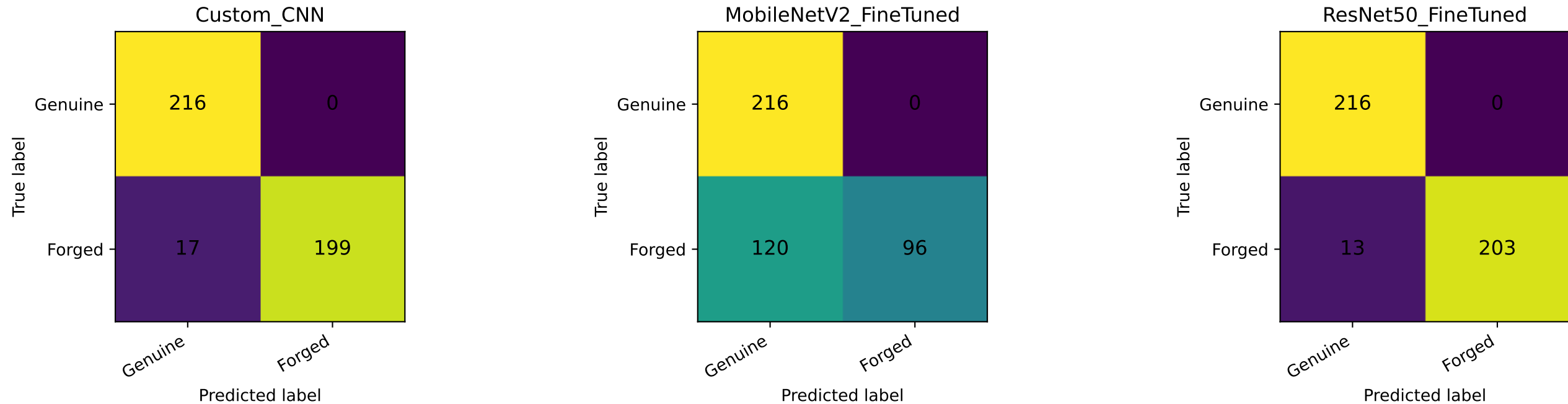
Figure 4. Confusion Matrix Comparison for Signature Verification Models
